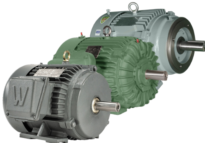
From Top to Bottom: Hyundai IEEE-841 Motor, WorldWide Electric Explosion Proof Motor, WorldWide Electric Premium Efficiency Severe Duty Motor
