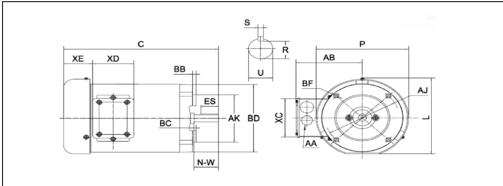
DIMENSION - INCHES
