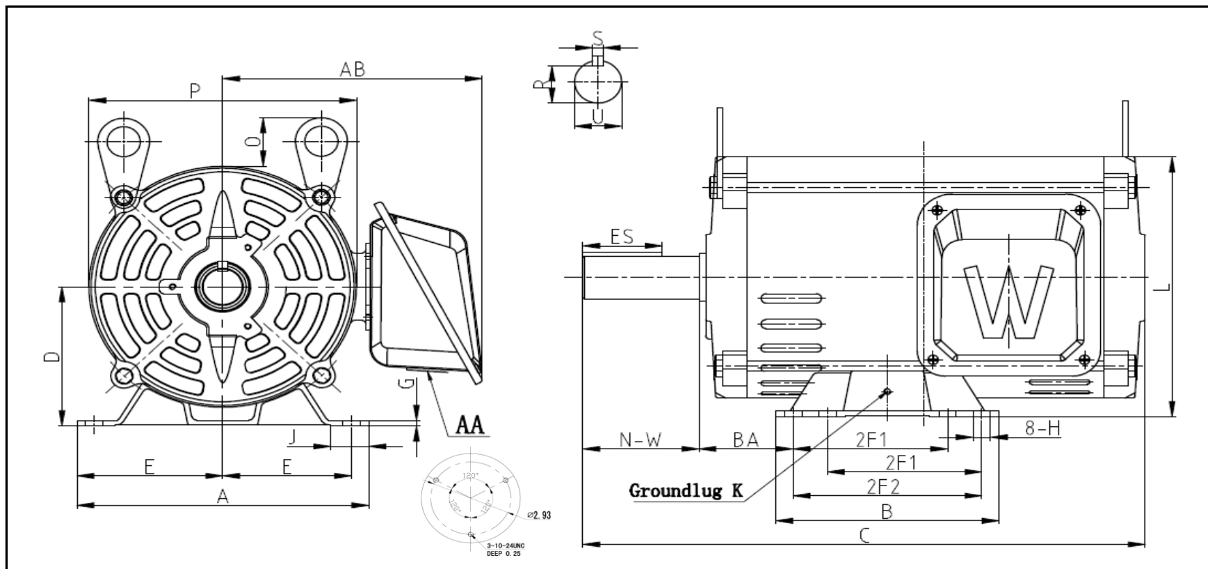
DIMENSIONS - INCHES
